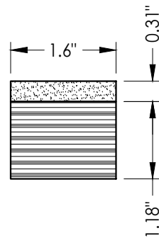
33 TOP RAIL
